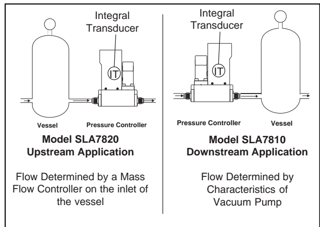
Figure 1 Typical Configurations
